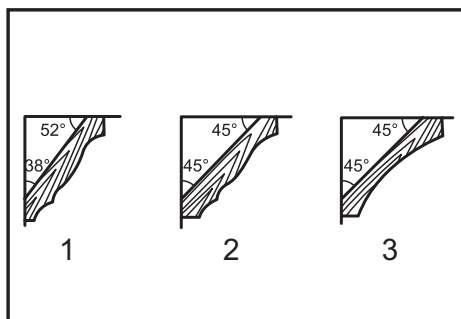
► 1. 52/38° type crown molding 2. 45° type crown molding 3. 45° type cove molding
